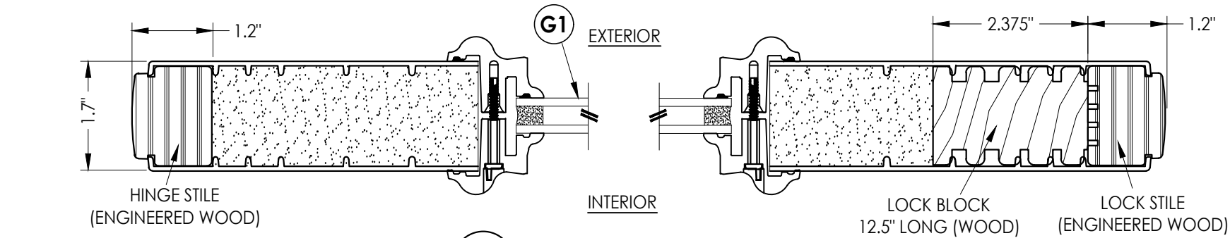
1 HORIZONTAL CROSS SECTION 2 WOOD EDGE
